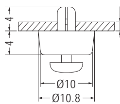
MOUNTING HOLE Ø3.6
