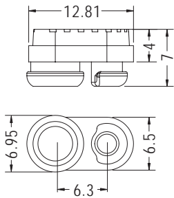
MOUNTING HOLE Ø5.6 CHASSIS THICKNESS 1.0-1.2
