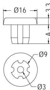
MOUNTING HOLE Ø8.3-Ø8.5
