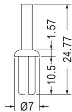
MOUNTING HOLE \varnothing 4.6 \sim \varnothing 4.8 THICKNESS 6.5
