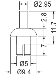
MOUNTING HOLE Ø5.1 THICKNESS 4.1~5.1
