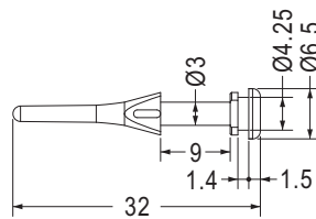
CHASSIS MOUNTING HOLE Ø4.4 CHASSIS THICKNESS 1.2
