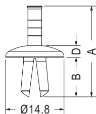
MOUNTING HOLE: \varnothing G THICKNESS: T
