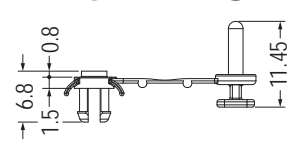
MOUNTING HOLE Ø4.0 THICKNESS 2.3-2.9
