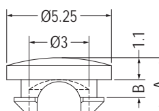
MOUNTING HOLE \varnothing 4.0 THICKNESS: T
