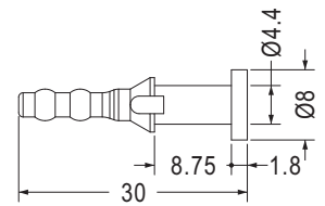
MOUNTING HOLE Ø4.4~Ø4.5
