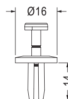
MOUNTING HOLE Ø7.0 THICKNESS 6.0
