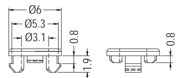
CHASSIS Ø5.3 THICKNESS 0.8
