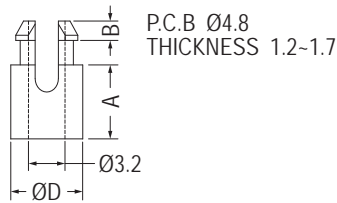
FOR M3 SCREW
