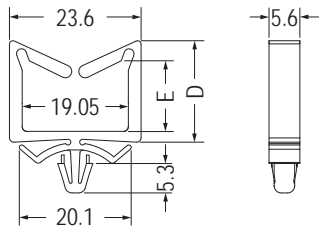
MOUNTING HOLE \varnothing 4.75 THICKNESS 1.2
