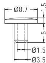
MOUNTING HOLE Ø3.5
