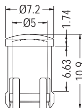
MOUNTING HOLE \varnothing 6.4 - \varnothing 6.45 THICKNESS 0.8-6.35
