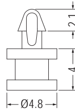
MOUNTING HOLE Ø2.0 THICKNESS 1.6
