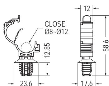
MOUNTING HOLE THICKNESS 0.6-6.75 (RECOMMEND FOR REFERENCE ONLY)
