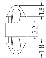
MOUNTING HOLE \varnothing 2.6 THICKNESS 1.0
