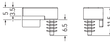
MOUNTING HOLE \varnothing 3.5
