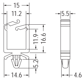
MOUNTING HOLE \varnothing 4.8 THICKNESS 0.8-1.8
