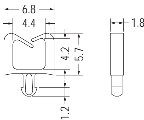
MOUNTING HOLE Ø1.75 THICKNESS 1.6
