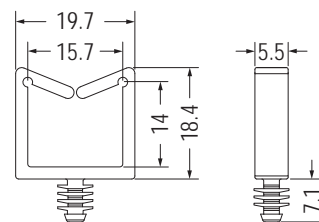
MOUNTING HOLE Ø5.3 THICKNESS 6.4
