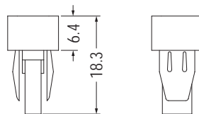
MOUNTING HOLE THICKNESS 0.8-2.0
