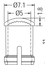
MOUNTING HOLE \varnothing 6.4 - \varnothing 6.45 THICKNESS 0.8-6.35
