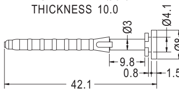
MOUNTING HOLE Ø4.4 THICKNESS 0.8~1.0
