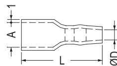
FLAT INSULATING SLEEVES
