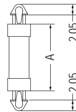
MOUNTING HOLE \varnothing 2.6 THICKNESS 1.6
