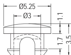
MOUNTING HOLE \varnothing 3.7 - \varnothing 3.8 THICKNESS 0.8-1.6
