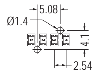
HOLE FOR P.C.B THICKNESS 1.6
