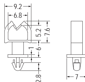
MOUNTING HOLE Ø3.0 THICKNESS 1.0-1.6
