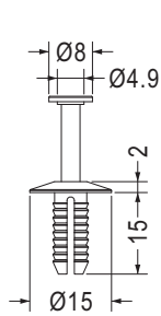
MOUNTING HOLE Ø6.35
