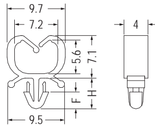
MOUNTING HOLE Ø3.0 THICKNESS 0.6~1.6
