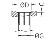
HOLE IN PANEL
