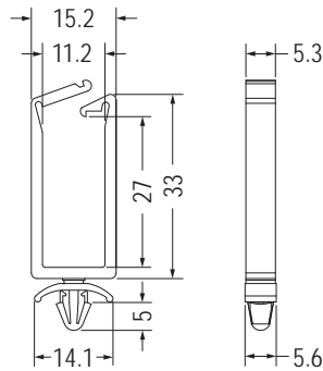
MOUNTING HOLE \varnothing 4.8 THICKNESS: T
