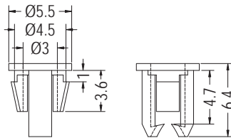
CHASSIS Ø4.5 THICKNESS 0.8
