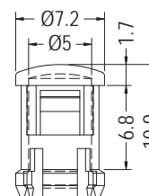
MOUNTING HOLE \varnothing 6.4 THICKNESS 0.8
