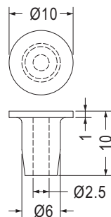
MOUNTING HOLE Ø5.5~Ø5.8
