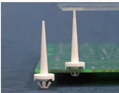
P.C.B Ø3.0 THICKNESS 0.65
