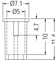
CHASSIS \varnothing 6.35 THICKNESS 0.8-1.4
