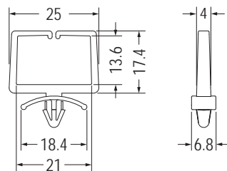
MOUNTING HOLE \varnothing 4.8 - \varnothing 5.0 THICKNESS 0.8-2.5
