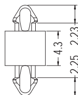
MOUNTING HOLE \varnothing 2.5 THICKNESS 1.6
