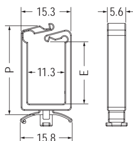
MOUNTING HOLE THICKNESS 0.8-1.6
