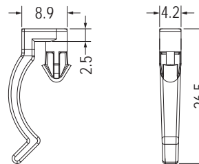
MOUNTING HOLE \varnothing 4.3 THICKNESS 4.0
