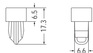
MOUNTING HOLE THICKNESS 2.0
