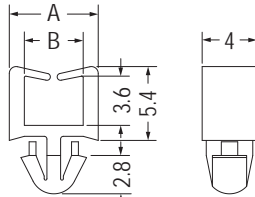
MOUNTING HOLE Ø3.5 THICKNESS: T
