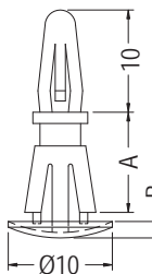
MOUNTING HOLE Ø5.5 THICKNESS 1.0-1.7
