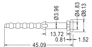
MOUNTING HOLE Ø5.1
