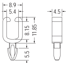
MOUNTING HOLE Ø4.0 THICKNESS 2.2
