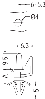
P.C.B Ø4.0 THICKNESS 1.6~1.8
