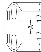
MOUNTING HOLE Ø2.5 THICKNESS 1.6
