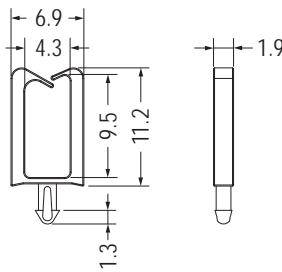
MOUNTING HOLE Ø1.75 THICKNESS 2.2
