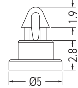
MOUNTING HOLE Ø2.0 THICKNESS 1.0
