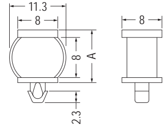
MOUNTING HOLE Ø3.0 THICKNESS 1.6
