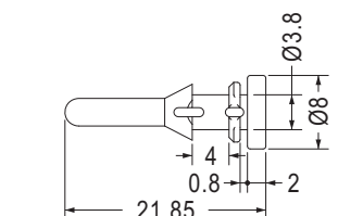
MOUNTING HOLE Ø4.4-Ø4.5 THICKNESS 0.8
