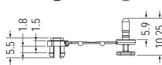
MOUNTING HOLE Ø4.0 THICKNESS 1.6
