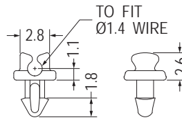
MOUNTING HOLE Ø2.0 THICKNESS 1.6
