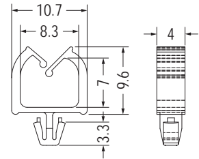
MOUNTING HOLE Ø3.3 THICKNESS 1.0
