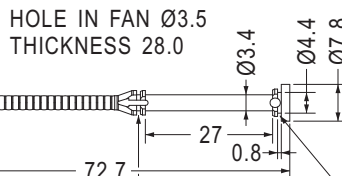
MOUNTING HOLE Ø3.5 THICKNESS 0.8
