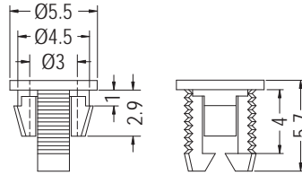
CHASSIS Ø4.5 THICKNESS 0.8
