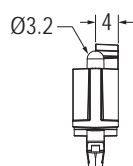
MOUNTING HOLE THICKNESS 2.2-2.5
