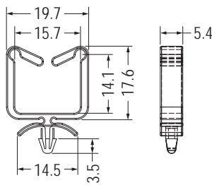
MOUNTING HOLE Ø3.0 THICKNESS 1.6~2.3
