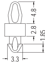
MOUNTING HOLE \varnothing 2.5 THICKNESS 1.6
