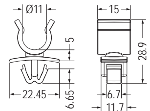
MOUNTING HOLE THICKNESS 3.0
