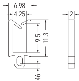
MOUNTING HOLE Ø2.8 THICKNESS 2.0
