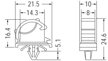
MOUNTING HOLE \text{\O}4.8 THICKNESS 0.8-2.5
