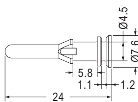
MOUNTING HOLE Ø4.5
