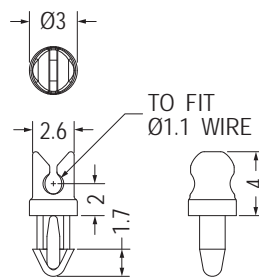
MOUNTING HOLE Ø2.0 THICKNESS: T
