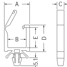
MOUNTING HOLE \varnothing 4.8 THICKNESS 0.5-2.0
