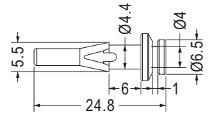
CHASSIS MOUNTING HOLE Ø4.0 CHASSIS THICKNESS 1.0
