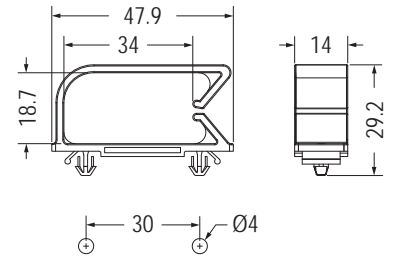
MOUNTING HOLE THICKNESS 0.8-2.0
