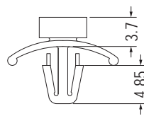
MOUNTING HOLE Ø4.0 THICKNESS 1.0-2.0
