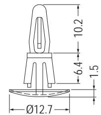
MOUNTING HOLE Ø5.4 THICKNESS 1.2-2.0
