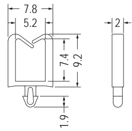
MOUNTING HOLE Ø2.0 THICKNESS: T
