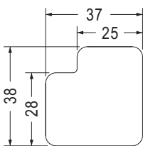
MOUNTING HOLE THICKNESS 2.0 (RECOMMEND FOR REFERENCE ONLY)
