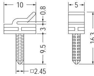
MOUNTING HOLE \varnothing 3.0
