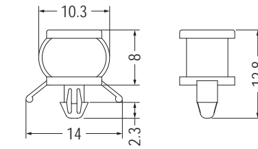
MOUNTING HOLE Ø3.0 THICKNESS 1.1-1.6
