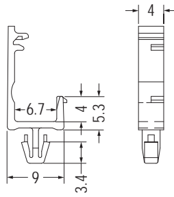
MOUNTING HOLE Ø3.0 THICKNESS 1.2-1.7
